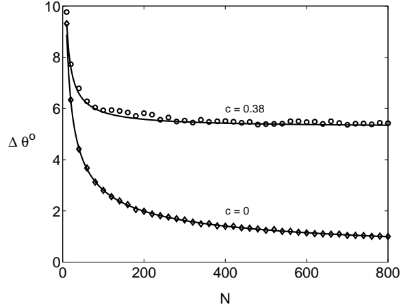
FIG. 6. Average error of the ML estimator and the Cramr-Rao bound as a function of the number of neurons, N , in the pool. The error of the ML estimator is nicely shown to saturate the bound. The error is represented in degrees. The parameters of the tuning curves are f_{\max} = 25 , f_{\text{ref}} = 5 and \sigma = \pi/4 , for the correlations a = 15 , c = 0.38 and \rho = 1 . The lower line corresponds to the error of the ML estimator for an independent population.
