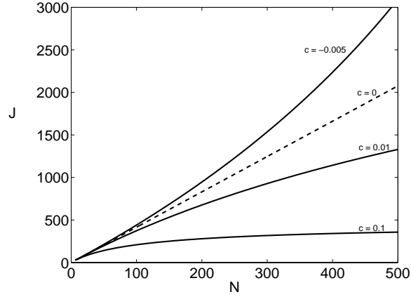
FIG. 3. Fisher Information of the population as a function of the number of neurons, N , in the pool. The linear curve (dashed line) represents J_o for independent population. J with negative correlation lies above J_o whereas with positive correlations lie below. For all cases, \rho = 1 , a = 15 , \sigma = \pi/4 , f_{max} = 25 and f_{ref} = 5 .
