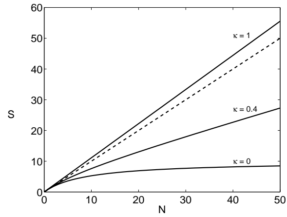
FIG. 1. Squared Signal to Noise Ratio as a function of the number of neurons, N , which are uniformly correlated with c = 0.1 . The dashed line represents the Signal to Noise Ratio of the independent population. The topmost curve is for \kappa = 1 , and from the bottom \kappa = 0 and \kappa = 0.4 .
