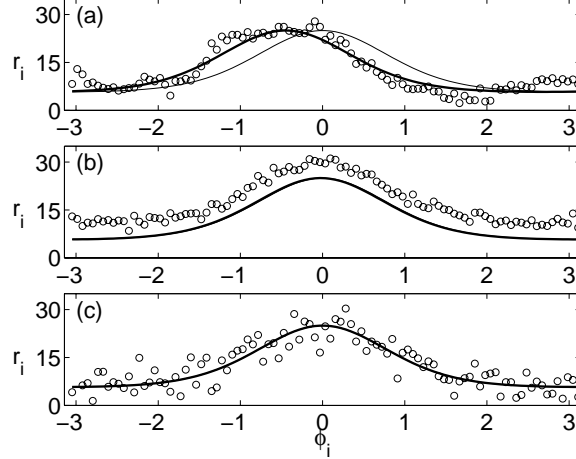
FIG. 5. Typical data generated according to Eq. (20) for a system with N = 100 neurons. Exponentially decaying correlations, Eq. (25), were used with: (a) \rho = 1.18 , (b) \rho \rightarrow \infty - uniform correlations and (c) \rho = 0 - independent population. Each circle represents the number of spikes of a single neuron in the population, during a 500msec time interval. The thick lines show f(\theta_{ML} - \phi_i) , where \theta_{ML} is the maximum likelihood estimate of \theta . The thin lines are the true mean responses of the neurons. Note that in (b) and (c) the thick and thin lines overlap. The parameters for the tuning curves are f_{\max} = 25 , f_{\text{ref}} = 5 , and \sigma = \pi/4 . The variance, a , was taken to be 15.
