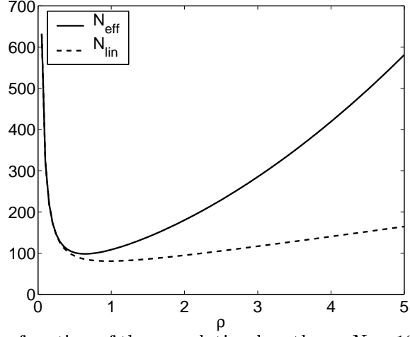
FIG. 4. N_{\text{eff}} and N_{\text{lin}} as a function of the correlation length, \rho . N = 1000 and c = 0.1 . Eq. (23)
