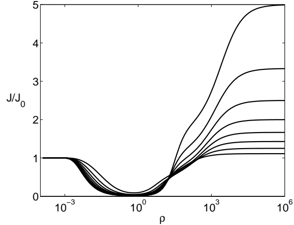
FIG. 2. Normalized Fisher Information as a function of correlation length, \rho . The correlation coefficient varies from c = 0.8 to 0.1 with a uniform spacing of 0.1 from the top to bottom when \rho is large. Eq. (23) was used for the tuning curves, with \sigma = \pi/4 , f_{max} = 25 and f_{ref} = 5 . The number of neurons, N , is 1000 . The ratio J/J_0 does not depend on the variance of
